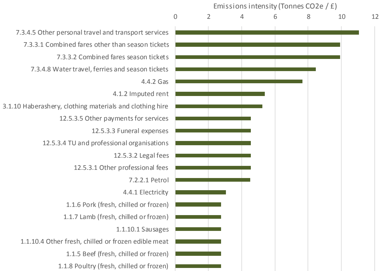
Chart 10. Conversion Factors: top 20 emissions intensities by product, 2017
