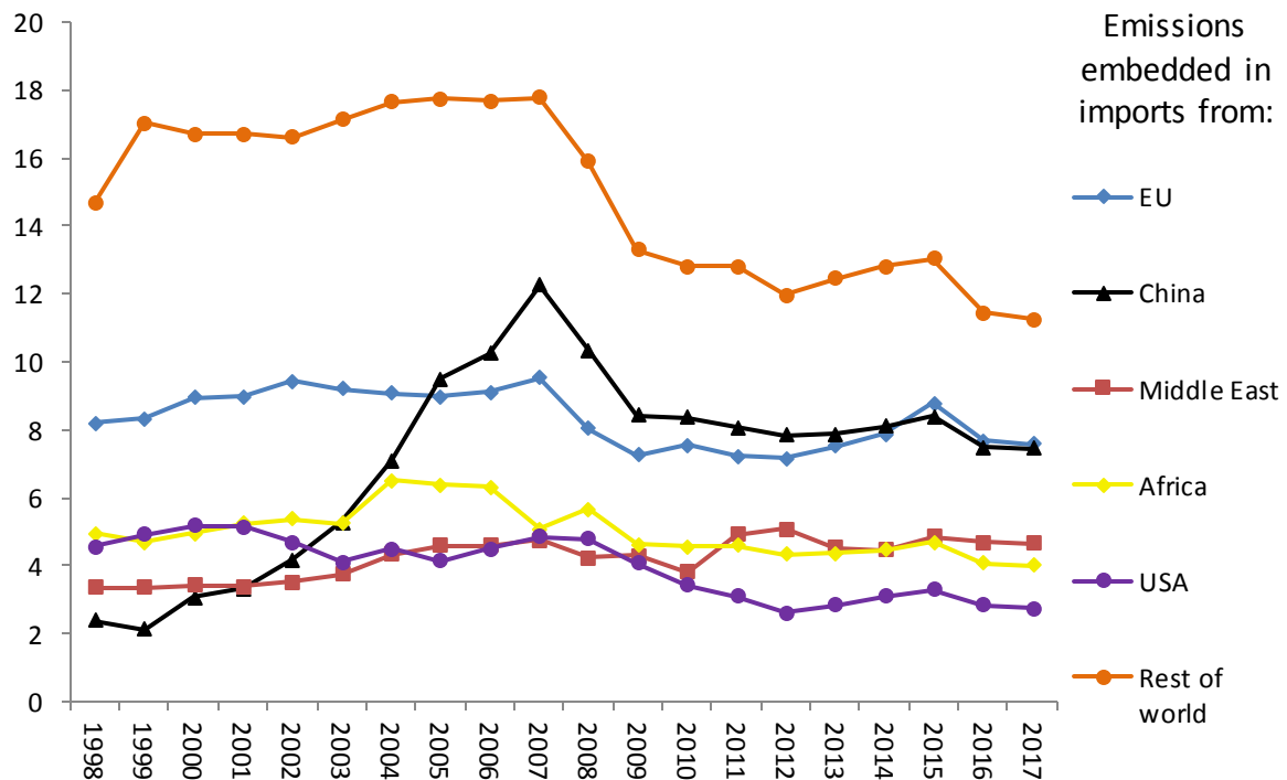
Chart 6. Breakdown of Scotland's embedded greenhouse gas emissions by region of import, 1998 to 2017. Values in MtCO 2 e
