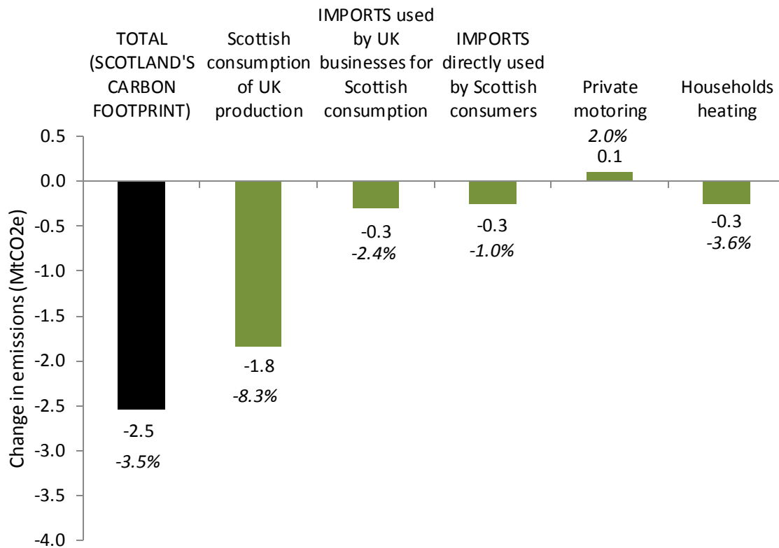
Chart 5. Change in Scotland's Carbon Footprint between 2016 and 2017 - in MtCO 2 e, and percentage changes
