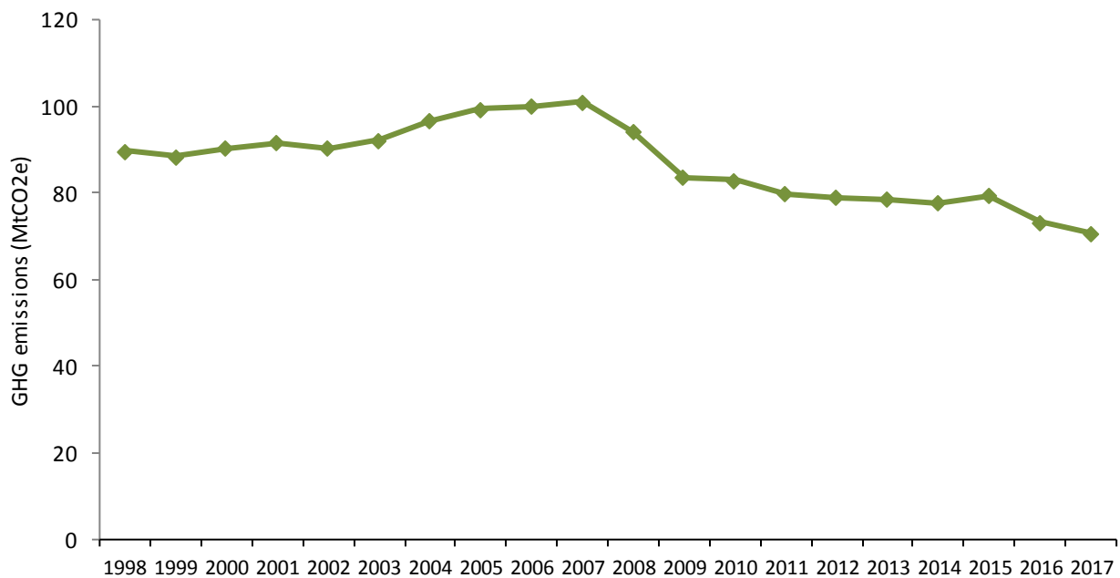
Chart 1. Scotland's Carbon Footprint, 1998-2017. Values in MtCO 2e
