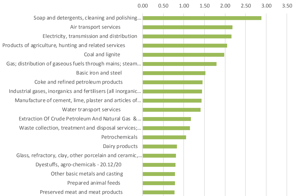
Chart 11. Total Impact Multiplier (UK): top 20 emissions intensities by product, 2017
