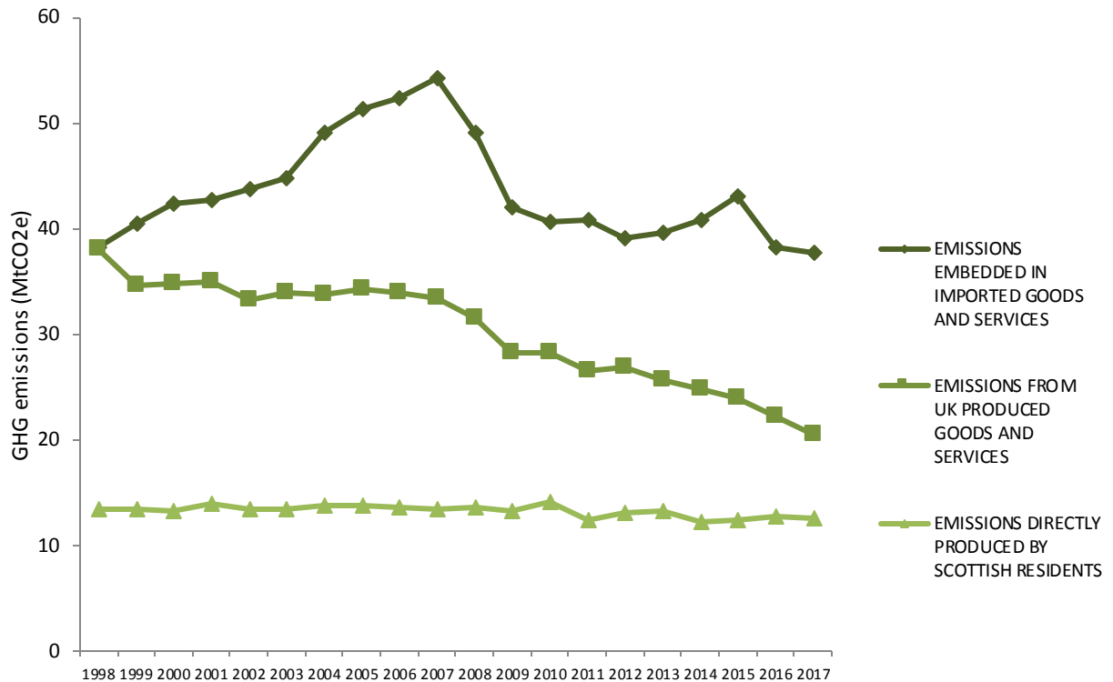
Chart 2. Scotland's Carbon Footprint, by main component, 1998 to 2017. Values in MtCO 2 e
