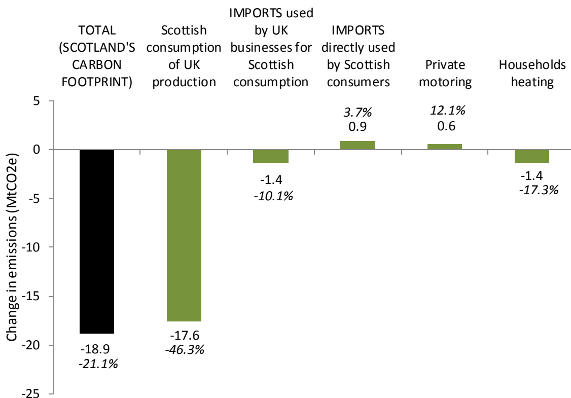
Chart 3. Change in Scotland's Carbon Footprint between 1998 and 2017 - in MtCO 2e , and percentage changes
