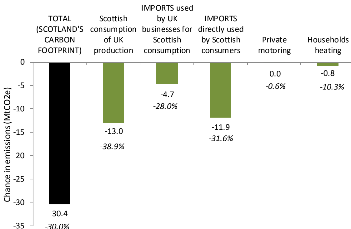
Chart 4. Change in Scotland's Carbon Footprint between 2007 and 2017 - in MtCO 2 e, and percentage changes
