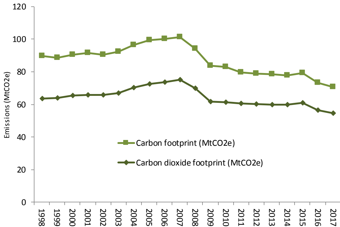
Chart 7. Scottish Carbon Footprint. Comparison of Carbon and CO 2 footprint. Values in MtCO 2 e
